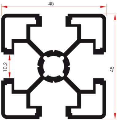
FSM 3001 1,404 kg/m
