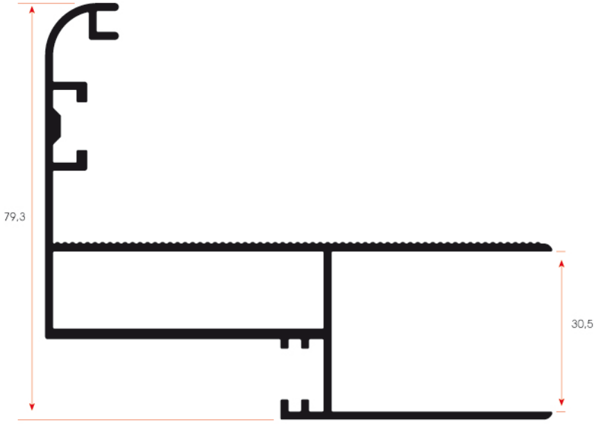
FSM 1500 1,500 kg/m
